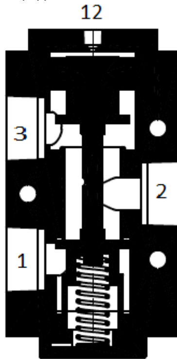
Figure 1 - 3/2 poppet valve series EP schematic diagram
